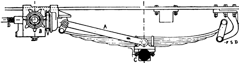
FIG. 76.—Spring and Radius Rod of the Mors Carriages. The rod, A, maintains a fixed distance between the sprocket pinion, B, and the wheel axle, C, even when the springs are constantly in action. This carriage also has a device for varying the distance between the countershaft at B, and the engine pulley, by sliding the entire shaft forward or back under impulse from the screw, D. The spring, being hung on links at front and rear, has considerable play, up and down, without disturbing the fixed relation of the axle, C, and the counter-shaft, B, as determined by the radius rod, A.
